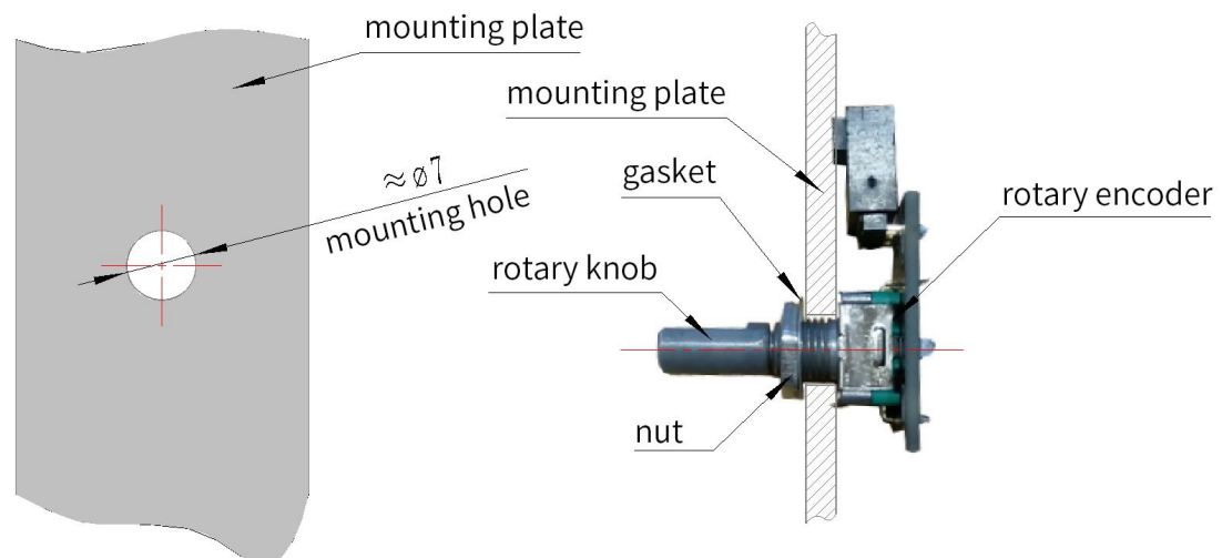
Figure 5-2 Nut Installation
