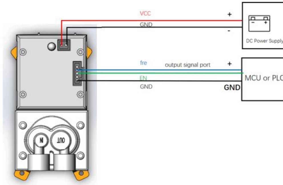
Figure 5-4 Wiring Diagram of Frequency Speed Control Type
