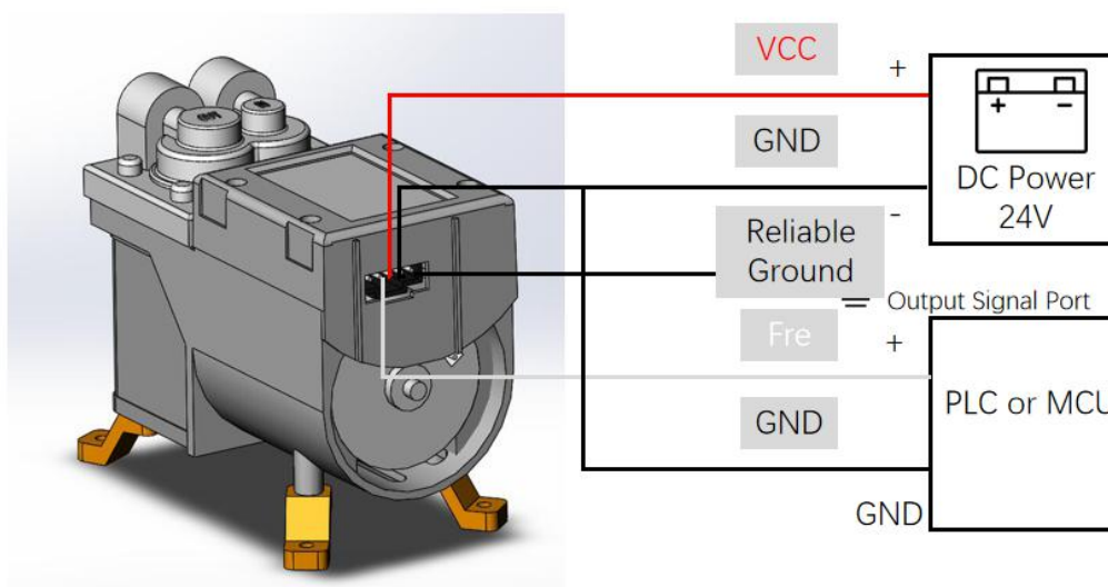
Figure 5-7 Wiring Instruction Using Frequency Speed Control
