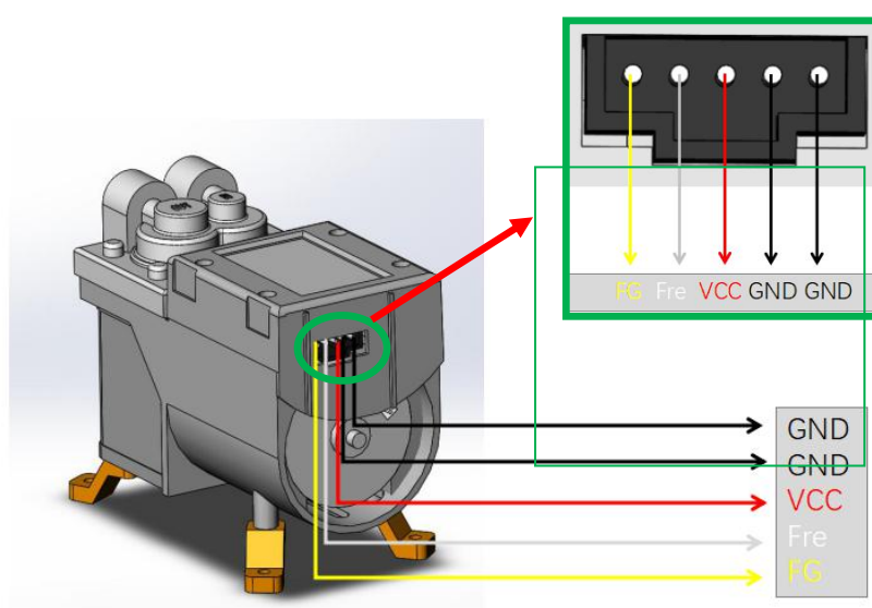
Figure 5-5 Description of Wire Terminal Signal of Top Configuration Type
