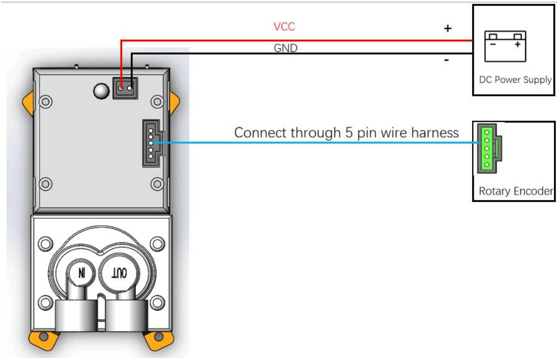
Figure 5-1 Wiring Diagram for Knob Speed Control Type
