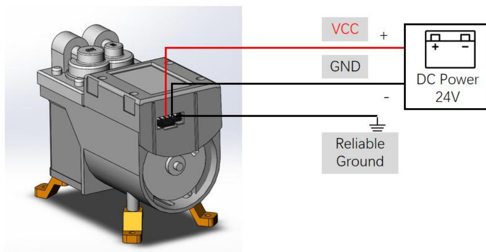
Figure 5-6 Wiring Instruction Using LCD Touchscreen
